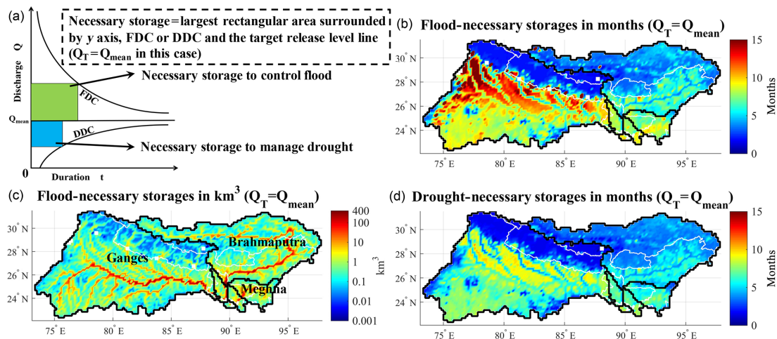
Figure 10. In nature, changes in the storage of water in a hydrological basin can smooth out hydrological variations associated with floods and droughts. The spatial variability in necessary hydrological storage, however, remains relatively unstudied – at the present time there is no global map showing the storage needed to ameliorate floods and droughts, either for the present climate or under climate change. Using the Ganges–Brahmaputra–Meghna Basin as an example, the needed storage at each grid cell within the basin is calculated with a new method: intensity–duration–frequency curves of flood and drought (flood duration curve and drought duration curve: FDC-DDC, an alternative representation of discharge time series obtained from a calibrated hydrological model called BTOPMC – see Takeuchi and Masood, 2016). For simplicity, the target release ( Q_T ) for smoothing is assumed to be the long-term mean discharge ( Q_{\text{mean}} ) at each grid cell (Takeuchi and Masood, 2016). The figure shows a typical FDC-DDC curve for a grid cell and an illustration of how to calculate necessary storage (a), the spatial distribution of storage (in units of \text{km}^3 ) needed to smooth floods in the basin (c), and the spatial distribution of storage (in units of months) needed to smooth flood (b) and drought (d). Note that storages expressed in months, calculated by dividing the necessary storage volume by the local Q_{\text{mean}} for 1979–2003, provide a unique perspective on storage requirements. The geographical distribution of necessary storage reflects hydrological heterogeneity associated with meteorological inputs, topography, geology, soil, vegetation, land use, and so on. Quantifying the relationships between spatially distributed necessary storages and the geographical distribution of hydroclimatological, geological, and land cover conditions can lead to improved hydrological analysis and produce useful information for water resources managers. (Contact: Muhammad Masood.)
