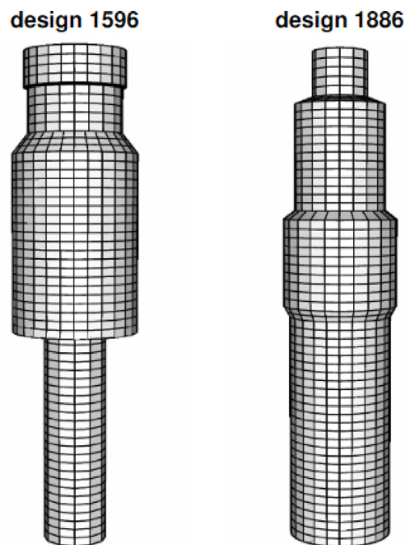
Fig. 7. SPAR support structure proposed in Birk and Clauss (2008).
