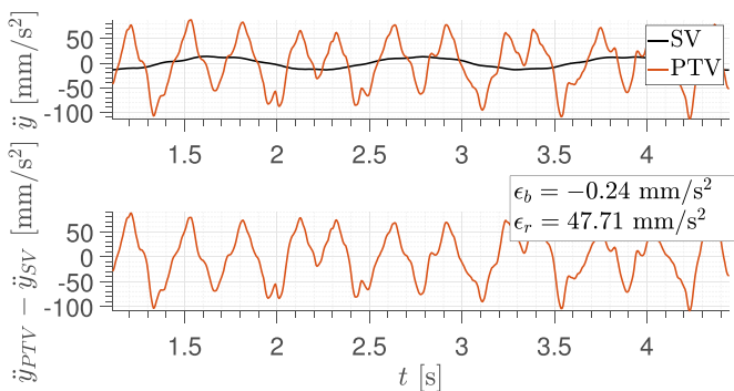
Figure C4. Time history of the instantaneous acceleration obtained from robotic volumetric PTV and SV measurements for the root marker (top) and of the related error (bottom). Only results from 3 gust cycles are shown.
