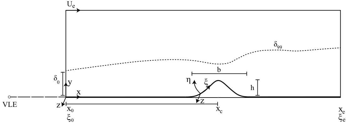
Fig. 1 Schematic of the problem showing the computational domain and coordinate systems, base flow, Virtual Leading Edge (VLE) and protuberance dimensions. (Note: the shown protuberance shape is only for illustration purposes, the exact shape is not shown)
