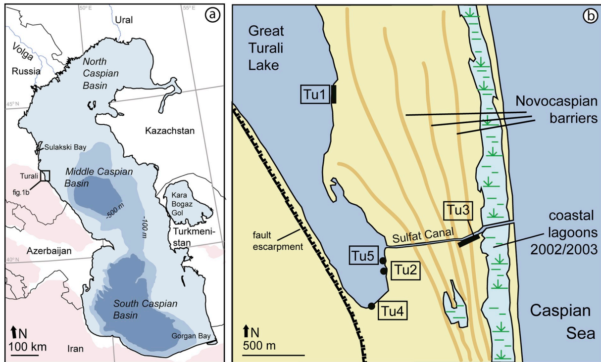
Fig. 1. Geographic context of study site. (a) Map of the Caspian Sea. Source bathymetry: Kostianoy et al. (2005): Fig. 1 (p. 7). (b) Location of the outcrops treated in this paper. Tu1-Tu5 represent outcrops Turali 1-5. Brown ridges are Holocene Novocaspian beach barriers (see Kroonenberg et al., 2007). (For interpretation of the references to colour in this figure legend, the reader is referred to the web version of this article.)
