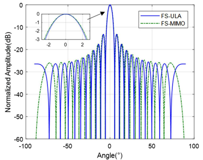
FIGURE 3 Array beam pattern comparison of FS-ULA and FS-MIMO in case 1: The 3 dB beam-widths are 4.84^{\circ} and 5.08^{\circ} , respectively. FS-MIMO, full-scale multiple-input multiple-output; FS-ULA, full-scale uniform linear array
