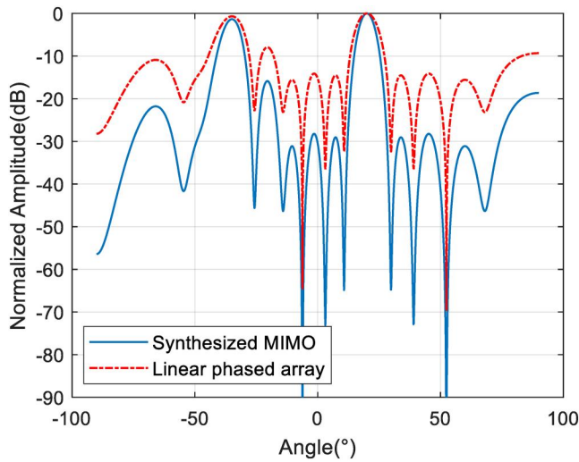
FIGURE 5 Optimised MIMO beam-pattern together with the physical T/R array beam-pattern (linear phased array) pointing at 20°: The side lobes near the MIMO beam-pattern main lobe ( \pm 40^\circ ) are under -28 dB, with one strong grating lobe located at 60^\circ away from the main lobe to the left. MIMO, multiple-input multiple-output; T/R, transmit–receive
