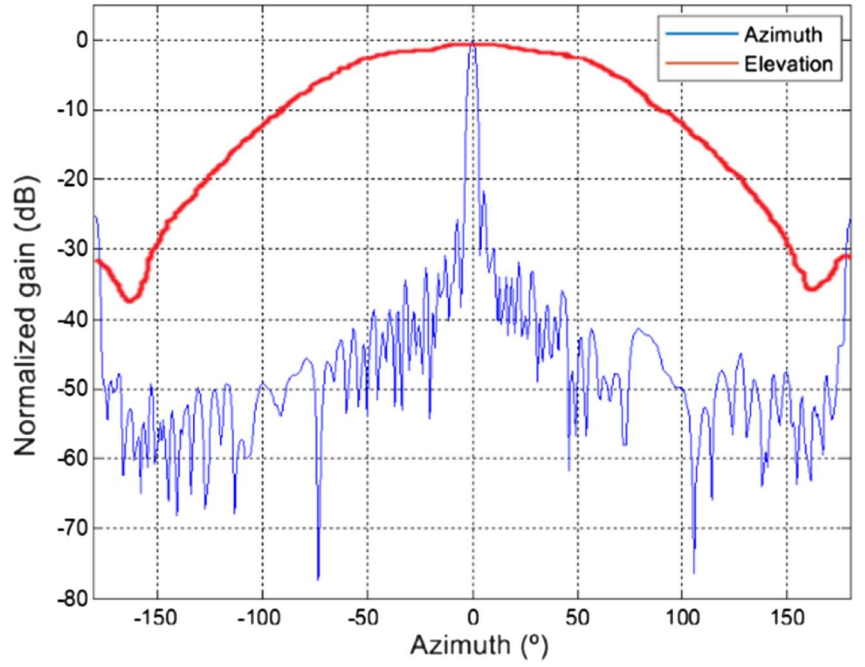
FIGURE 7 Radar antenna radiation pattern: with a beam-width of 3^\circ in azimuth and 110^\circ in elevation
