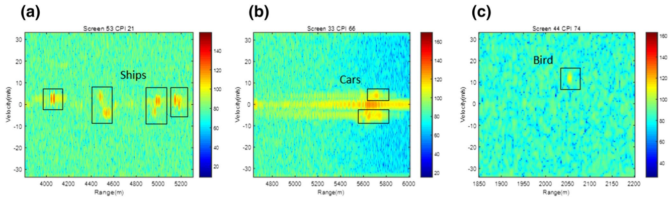
FIGURE 17 Range-velocity plane of other different targets: (a) ships on the river, (b) cars on the bridge, (c) birds. CPI, coherent processing interval
