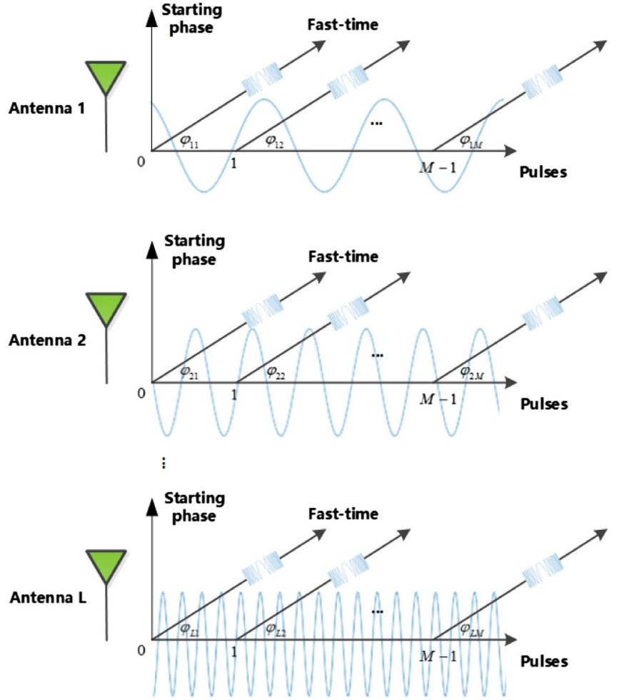
FIGURE 1 DDMA waveform signal model with L antennas: DDMA waveform adds different starting phase values to different pulses and channels intentionally, so that each channel has a unique Doppler shift. The intrapulse modulation can be the same for every pulse, for example a chirp. DDMA, Doppler division multiple access
