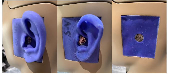
Fig. 4. KEMAR large anthropometric pinna replica (left), pinna replica of artificial head S (center), and silicone baffle (right) mounted on the KEMAR's left channel.
