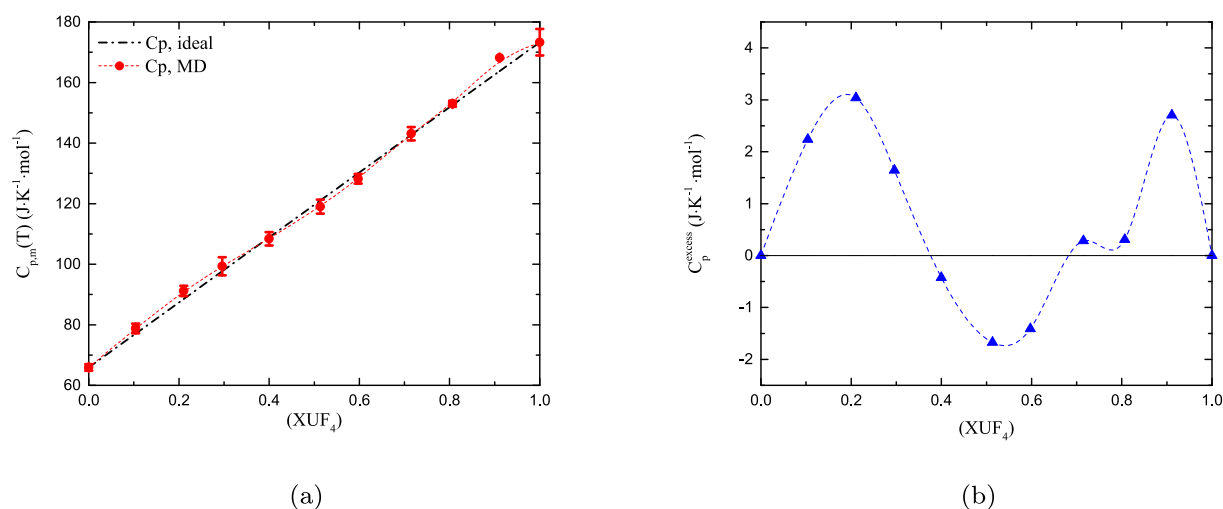
Fig. 12. (a) Heat capacity of the (\text{Li,U})\text{F}_x solution as calculated via MD (red) in the 900–1400 K temperature range, compared to the ideal heat capacity (black dashed line) obtained from the experimental heat capacities of the end-members (see Table 4 also). (b) Excess heat capacity of the (\text{Li,U})\text{F}_x solution derived from MD simulations.
