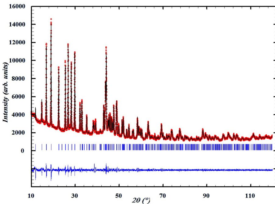
Fig. 4. Diffractogram of \text{LiUF}_5 , X(\text{UF}_4) = 0.5 . Comparison between the observed ( Y_{obs} , in red) and calculated ( Y_{calc} , in black) X-ray diffraction patterns. Y_{obs} - Y_{calc} , in blue, is the difference between the experimental and calculated intensities. The Bragg's reflection angular positions are marked in blue.
