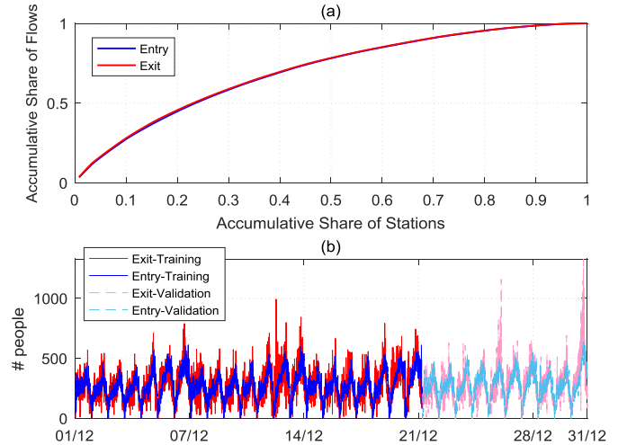
Fig. 2. Illustrations of flow profiles. (a) Cumulative distribution function plots of entry and exit flows; (b) A typical example of entry and exit flow time series of Shenzhen metro station (Luohu station).
