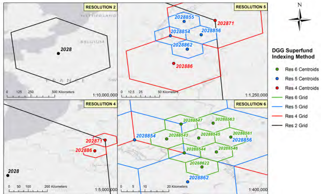
Figure 2.19: Relation between the indexes of the hexagons in resolutions 2, 4, 5 and 6 while using the DGG type Superfund_500m .
