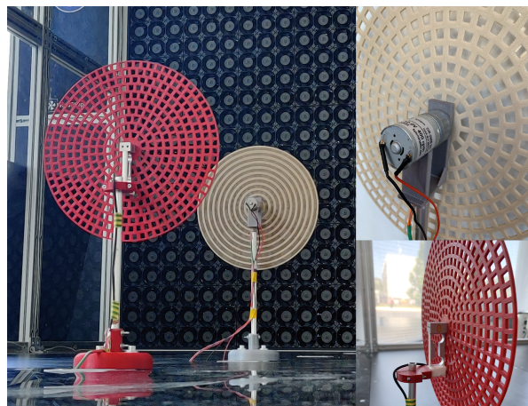
Figure 5: The test set-up as used in the Windshaper with the Helix porous disc (white) mounted at 5D upstream of the sensor porous disc (red). The top right image shows the DC motor used in the experiment. The bottom right image shows the load-cell and its mounting hardware.
