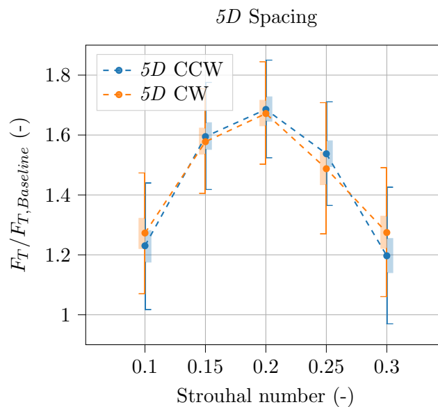
Figure 7: Thrust output of the downstream turbine for 5D spacing measured in a range of different Strouhal numbers. Each point represents the thrust averaged over 120s and normalised w.r.t the baseline.
