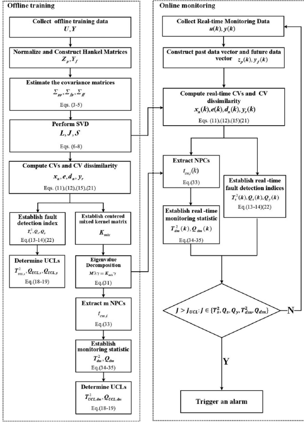
Fig. 2. Procedure of the proposed CVD-MKPCA based fault detection.
