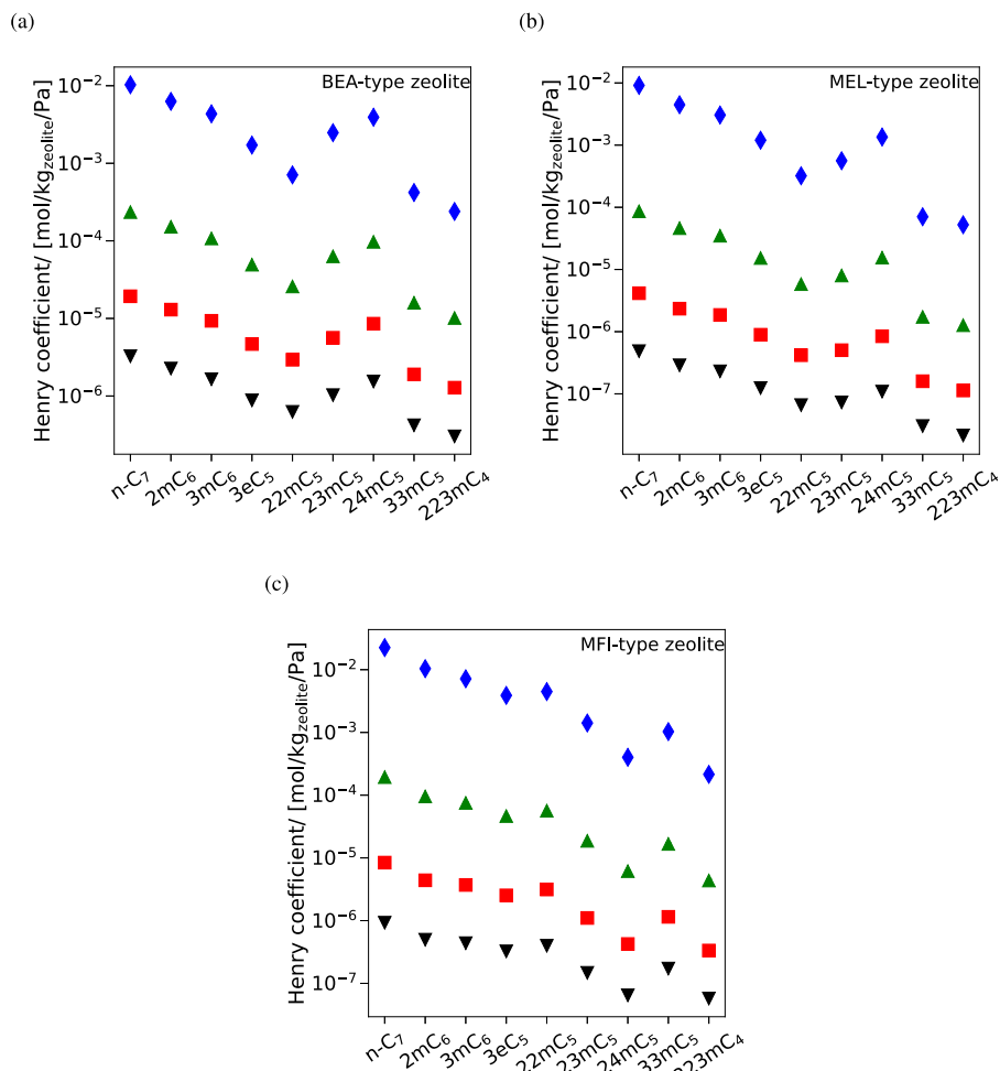
FIG. 5. Henry coefficients of C_7 isomers in (a) BEA-, (b) MEL-, and (c) MFI-type zeolites at 400 K (blue filled rhombus), 500 K (green filled triangle), 600 K (red filled square), and 700 K (black filled inverted triangle). The raw data are listed in the worksheets xi_iC7_400 K, xi_iC7_500 K, xi_iC7_600 K, and xi_iC7_700 K of the supplementary material , SI2.xlsx.
