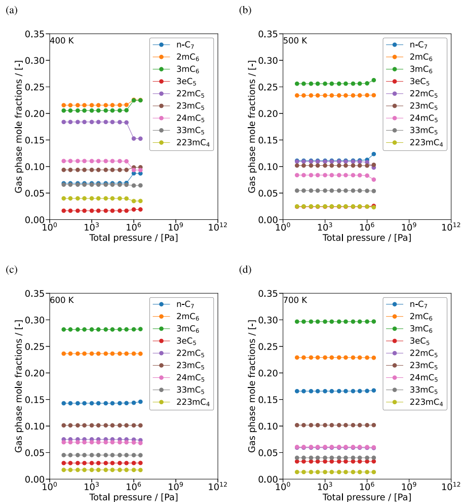
FIG. 13. Effect of gas phase pressure on the equilibrium distribution of C_7 isomers at temperatures (a) 400 K, (b) 500 K, (c) 600 K, and (d) 700 K. The raw data are listed in the worksheet InQ_ic7_high_press of the supplementary material , SI2.xlsx .
