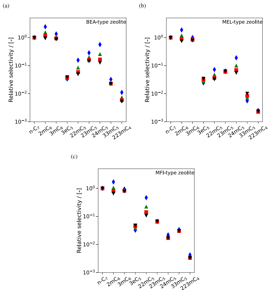
FIG. 10. Relative selectivities of different C_7 isomers at reaction equilibrium in (a) BEA-, (b) MEL-, and (c) MFI-type zeolites at infinite dilution. The reaction equilibrium distribution is computed at 400 K (blue filled rhombus), 500 K (green filled triangle), 600 K (red filled square), and 700 K (black filled inverted triangle). The raw data are listed in the worksheets xi_ic7_400 K , xi_ic7_500 K , xi_ic7_600 K , and xi_ic7_700 K of the supplementary material , SI2.xlsx.
