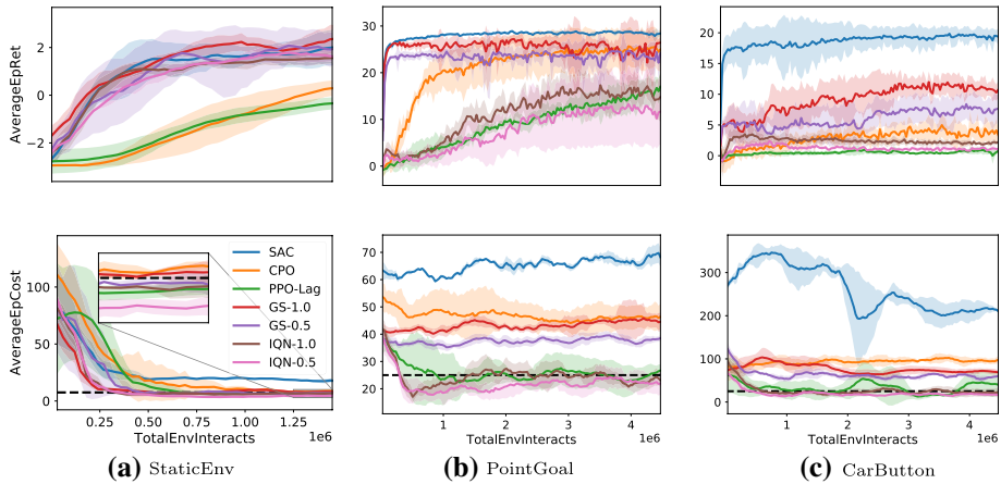
Fig. 10 Performance of the algorithms during training in terms of mean (solid lines) and \pm 1 standard deviation (shaded area) of the runs within an epoch. The black dashed lines indicate the safety thresholds
