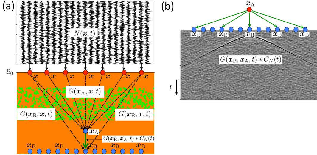
Figure 4. Principle of seismic interferometry. (a) Propagation of ambient noise from S_0 through an inhomogeneous medium to receivers at x_A and x_B . (b) Cross-correlation of responses at x_A and x_B (with x_A fixed and x_B variable).
