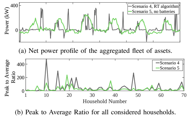
Fig. 9: Impacts of Scenario 4 and 5 on the grid.
