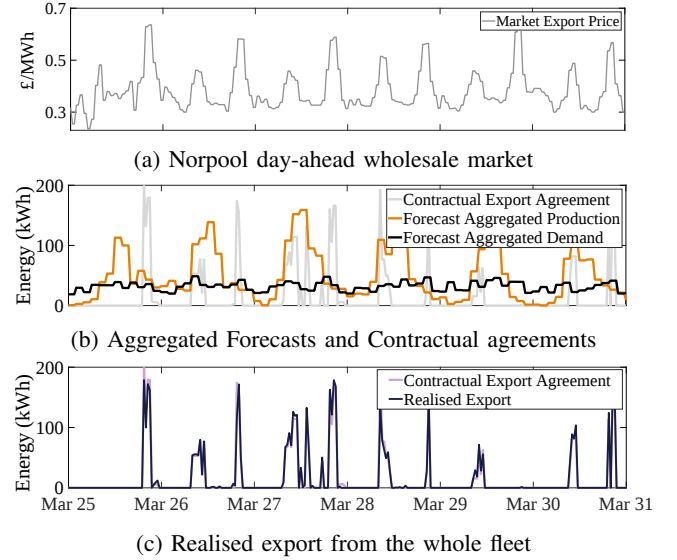
Fig. 5: Experimental results with 30 minutes time intervals
