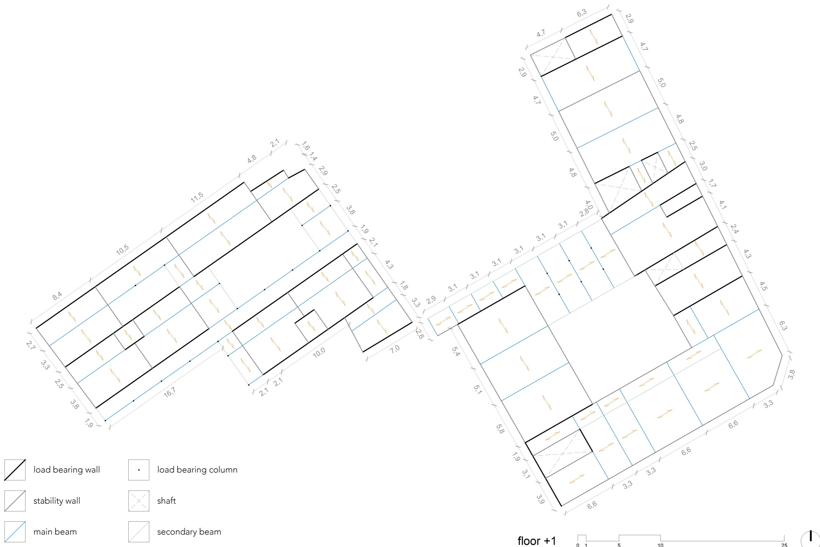
construction plan
