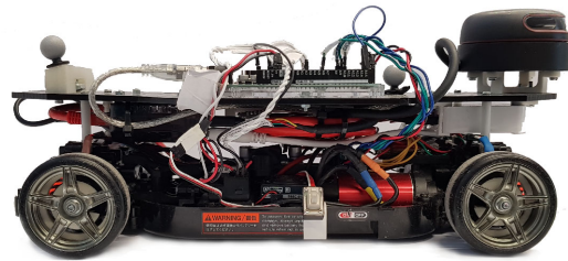
Fig. 15. The Delft Scaled Vehicle.
