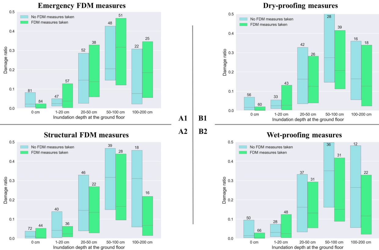
Figure 2. Depth-damage relationship for building structure, differentiated for the groups without flood damage mitigation (FDM) (blue) and with FDM (green) divided into emergency (A1) versus structural (A2) and dry- (B1) and wet-proofing (B2) FDM categories. The lower and upper parts of the boxes represent the 25th and 75th percentile of flood damage ratios, with the median in between. The number of observations on top of the boxes. Note. The group with FDM measures (green) only reflects the group that has taken FDM measures reflected in the figure. The group without FDM (blue) did not take that specific measure but may have taken other FDM measures.
