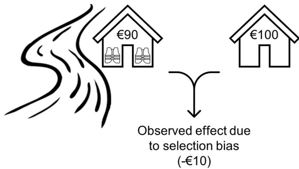
Figure 1. Selection bias that results in an underestimation of the true effect of flood damage mitigation (FDM) measures. Note. The building closest to the river faces higher flood risk (€120 vs. €100 in the top hypothetical situation without FDM measures) and is, therefore, more likely to take FDM measures (as shown in the actual situation below). However, we only observe the actual situation below where flood damage has occurred which implies an incorrect damage reduction of €10 (€100 vs. €90). The true effect of FDM measures is the difference between the counterfactual (hypothetical) situation without FDM measures (€120) and the observed situation (€90) with FDM measures: the damage reduction of FDM is €30. The buildings on the right are, therefore, not representative as control group, which results in an underestimation of the true effect of FDM measures.
