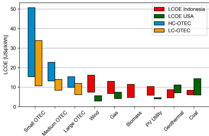
Fig. 5. OTEC’s competitiveness against other energy technologies in Indonesia in 2019. Small OTEC < 20 MW, medium OTEC 20 MW < P_{net} < 75 MW, large OTEC 75 MW < P_{net} < 100 MW. Gas includes open-cycle, closed-cycle, and combined-cycle. Coal refers to subcritical plants. LCOE of competing technologies based on [48] in Indonesia and based on [49] in USA.
