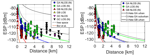
(a) Free-space and Bor models. (b) Okumura-Hata model.
