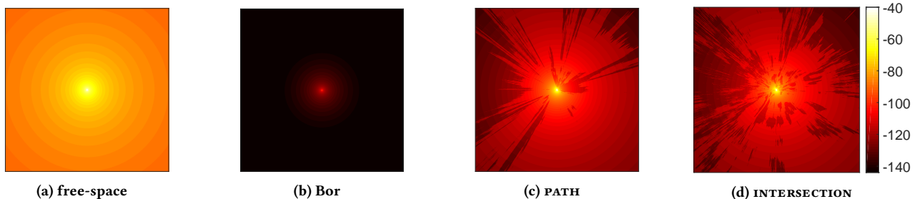
Figure 19: ESP prediction on a 6 \times 6 \text{ km}^2 area centered in G_8 .
