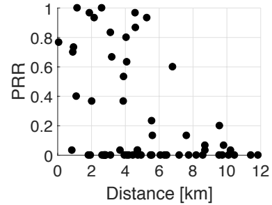
Figure 6: Link reliability (PRR) vs. distance for three gateways. LoRa provides only a single, long transitional region.
