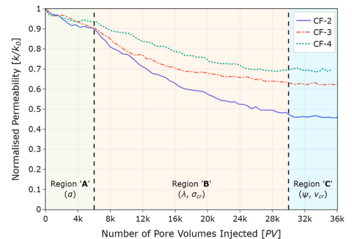
Fig. 22. Injectivity decline versus pore volumes injected for CF-2, 3 and 4 with the three distinctive decline regions. Horizontal axis is in thousands of PV injected.
