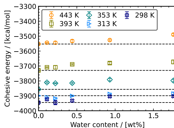
Fig. 13. Cohesive energy of bitumen components as a function of water contents at various temperatures.
