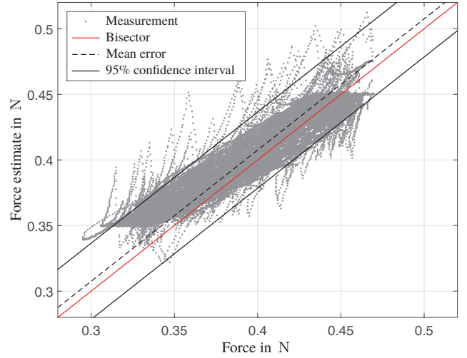
(b) Force estimation during force control.
