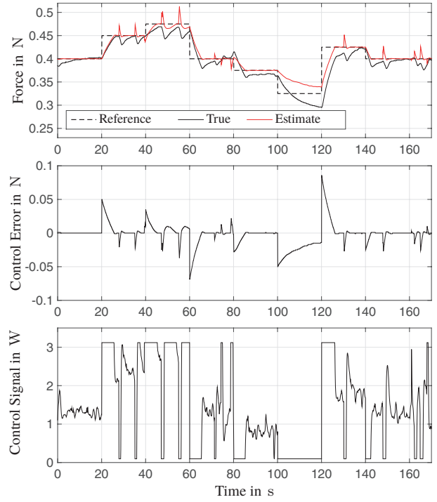
(b) Step response during force control.
