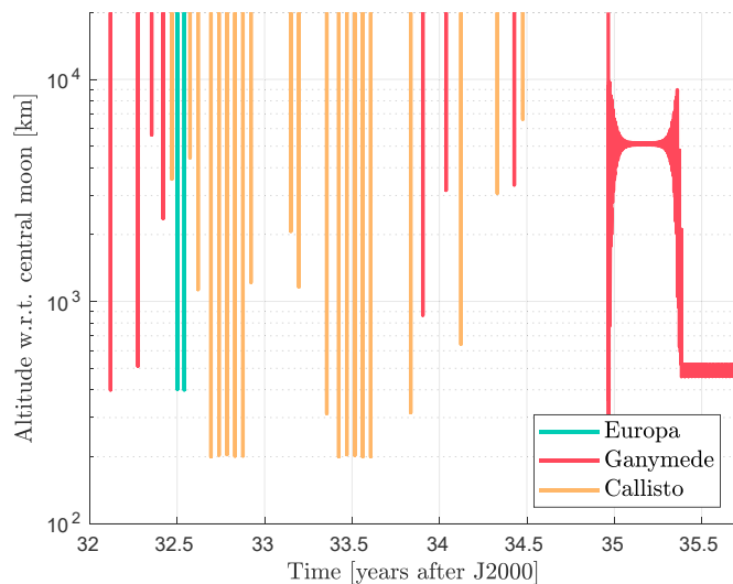
Fig. 1. Altitude of the JUICE spacecraft with respect to the Galilean moons during the flyby and orbital phases, based on CReMA 5.0. The vertical lines directly provide the closest-approach distances for the flyby series, while the orbit of JUICE around Ganymede is clearly identifiable, starting slightly before 2035.
