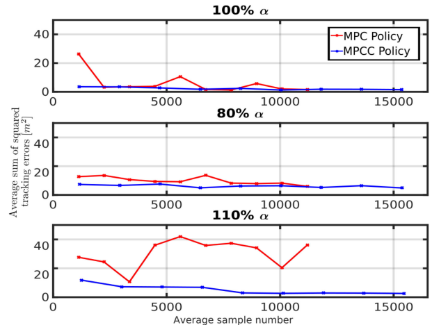
Fig. 9. Policy robustness : Policy performance as a function of the supervisor. The average error from three trained policies are shown. The error is bounded to 50. From experiments, we found that error below 10 gives satisfactory performance. Lower is better.
