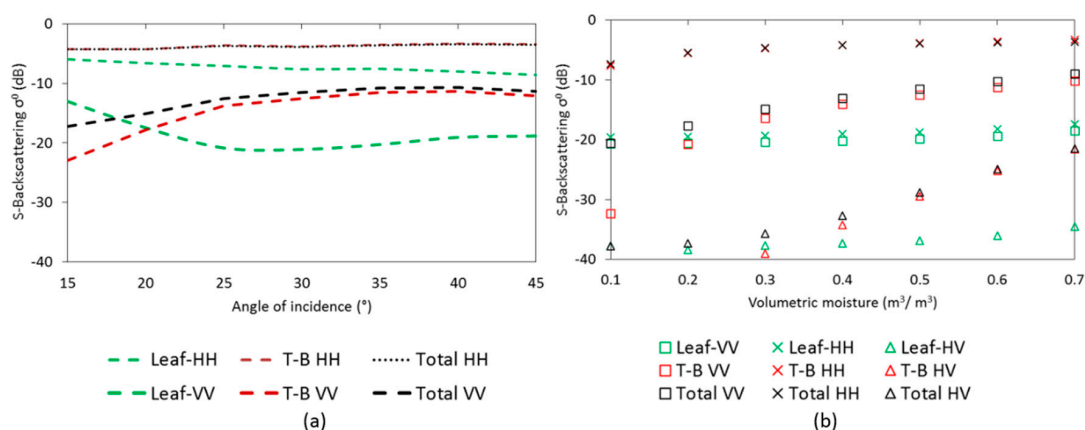
Figure A1. S-band backscatter vs. canopy parts (a) at 0.5 volumetric moisture ( m^3/m^3 ) across incidence angles and (b) at varying volumetric moisture ( m^3/m^3 ) at 30^\circ radar range where T- and B- represents trunk and branches respectively.
