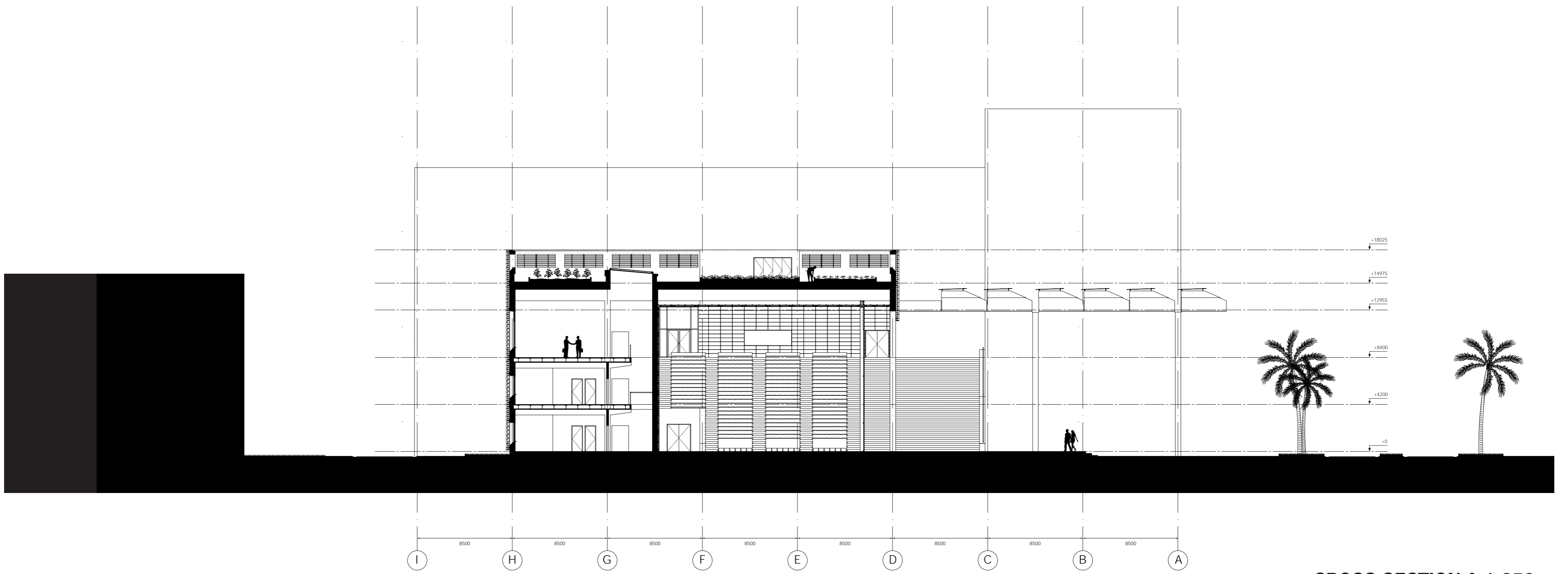
CROSS SECTION A 1:250
