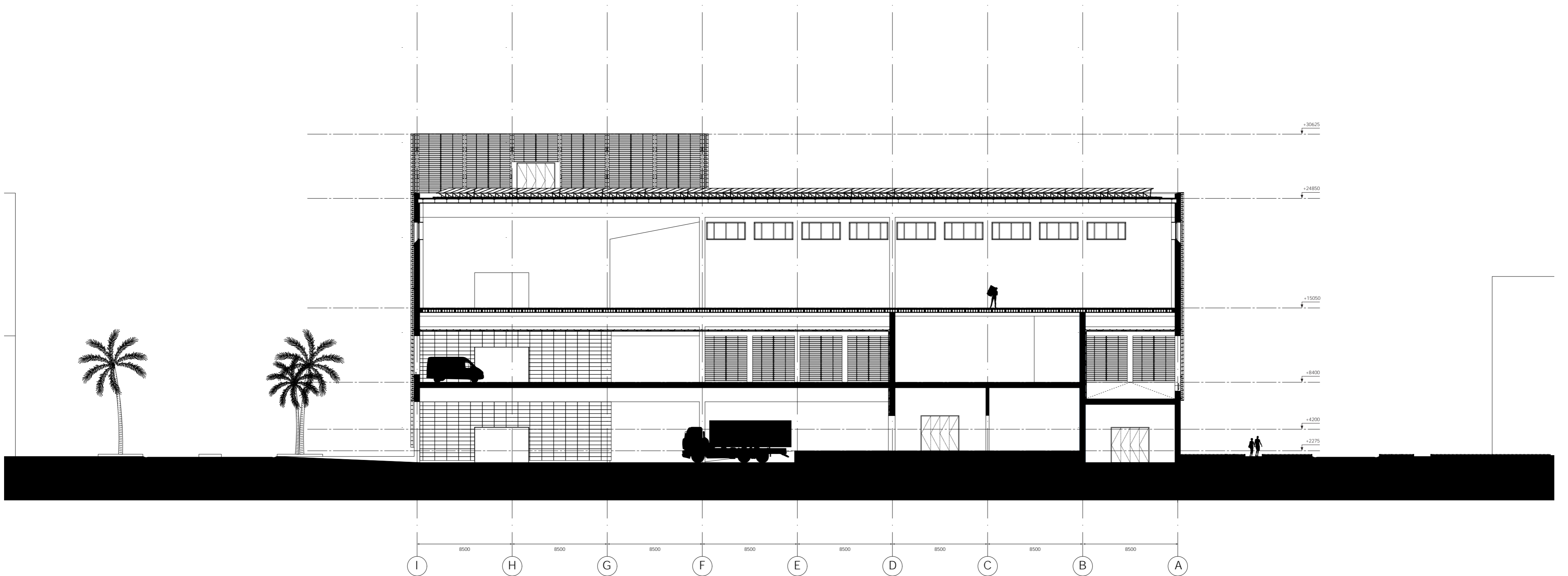
CROSS SECTION B 1:250
