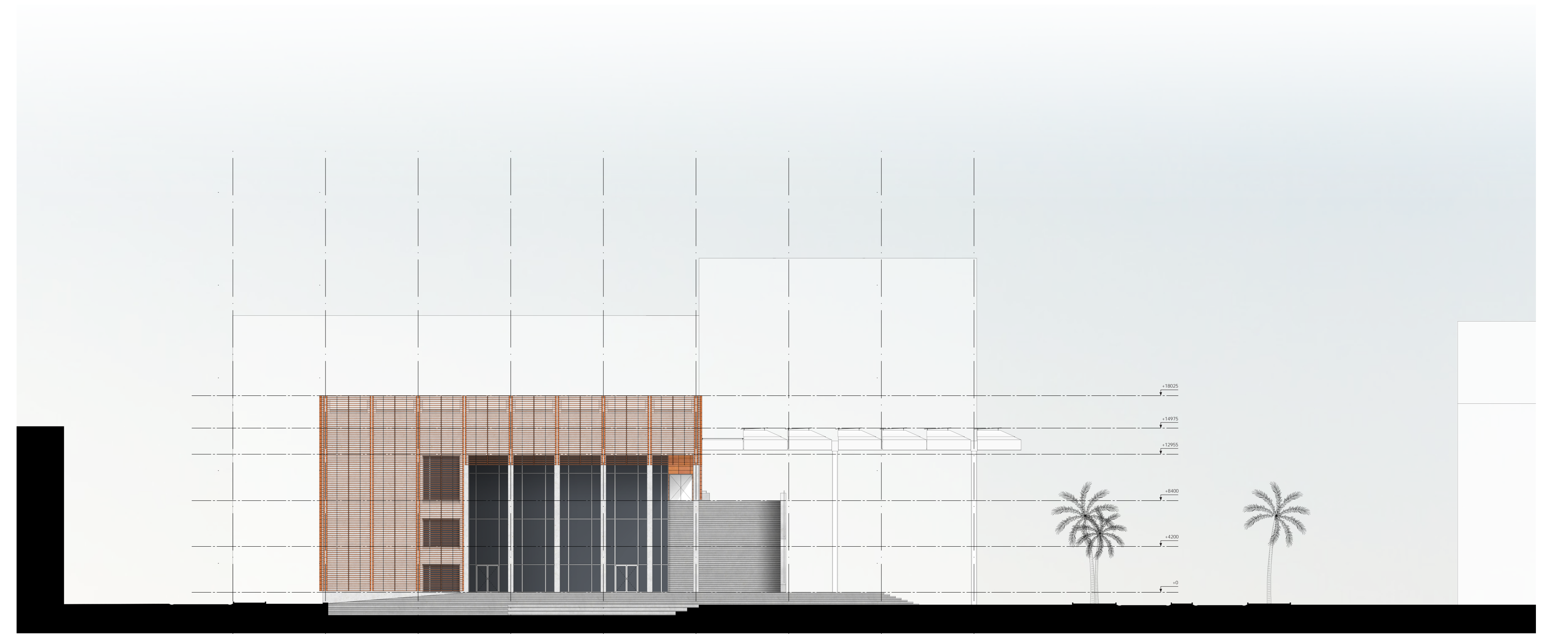
ELEVATION NORTH-EAST 1:250
