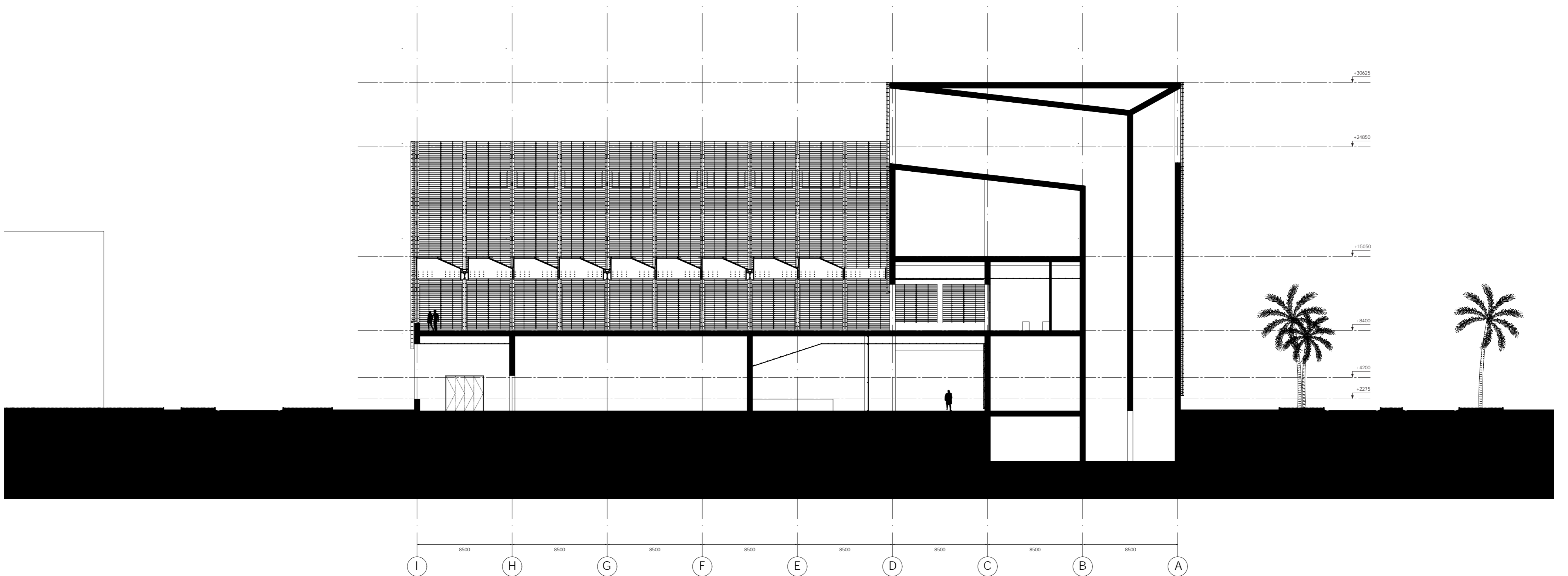
CROSS SECTION C 1:250
