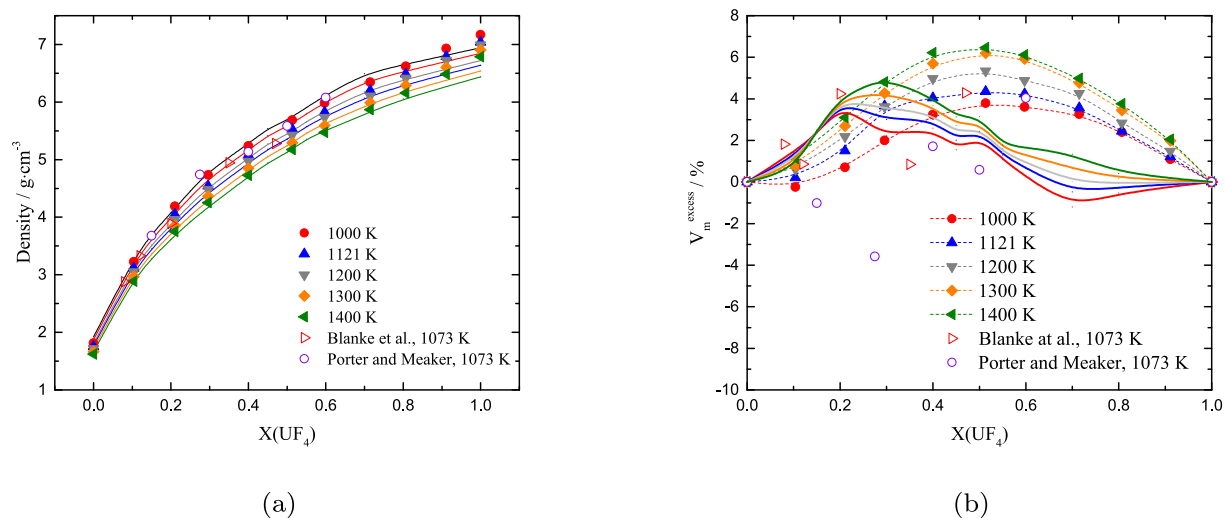
Fig. 11. Evolution of density. (a) Solid lines: isotherms calculated from the empirical equations reported by Klimentkov et al. [67]; solid symbols: results derived from MD simulations; ▶, red, experimental data by Blanke et al. [68] and ○ (purple) by Porter and Meaker [69], T = 1073 K. (b) Relative excess molar volume (%), of the (Li,U)F x solution.
