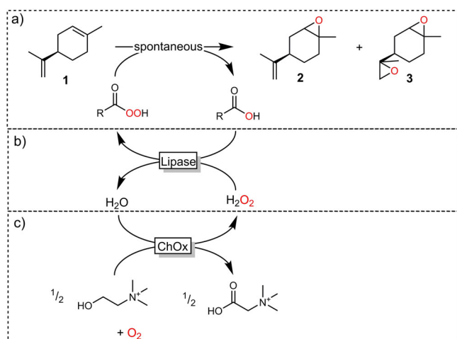
Scheme 1. Biocatalytic cascade epoxidation of limonene. a) Direct oxidation of limonene into limonene epoxide enabled by peracids. b) Formation of peracids catalyzed by lipase with \text{H}_2\text{O}_2 . c) Formation of \text{H}_2\text{O}_2 enabled by ChOx-catalyzed choline chloride oxidation in NADES and \text{O}_2 reduction.
