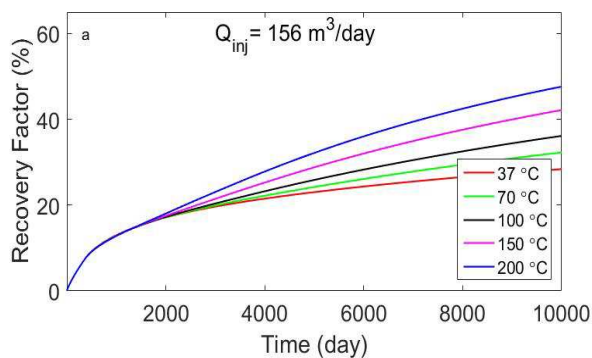
Figure 10: Recovery factor for different injection temperature and injection rates: a) 156 m 3 /day b) 318 m 3 /day.
