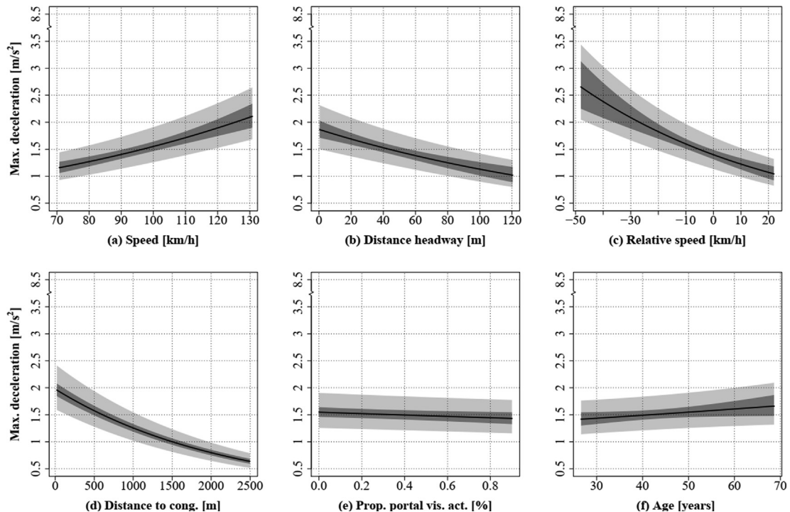
Fig. 2. Impact of the continuous explanatory variables on the maximum deceleration during the event. Black solid lines denote the marginal means, dark grey ribbons indicate the 95% confidence intervals, and light grey ribbons denote the 95% prediction intervals. The variables are listed as follows: (a) speed, (b) distance headway, (c) relative speed, (d) distance to the beginning of congestion, (e) proportion of time when the portal is visible and active, (f) driver age. The axis scales are chosen based on the minimum and the maximum values available in the data. To improve the readability, the vertical axis is interrupted at maximum deceleration equal to 3.75 m/s 2 .
