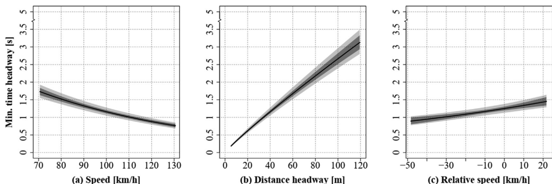
Fig. 4. Impact of the continuous explanatory variables on the minimum time headway during the event. Black solid lines denote the marginal means, dark grey ribbons indicate the 95% confidence intervals, and light grey ribbons denote the 95% prediction intervals. The variables are listed as follows: (a) speed, (b) distance headway, (c) relative speed. The axis scales are chosen based on the minimum and the maximum values available in the data. To improve the readability, the vertical axis is interrupted at minimum time headway equal to 3.75 s.
