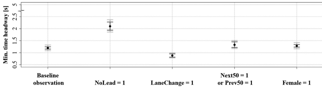
Fig. 5. Impact of the nominal explanatory variables on the minimum time headway during the event. Black dots denote the marginal means, dark grey error bars indicate the 95% confidence intervals, and light grey error bars denote the 95% prediction intervals. The vertical axis scale is chosen based on the minimum and the maximum values available in the data. To improve the readability, the axis is interrupted at minimum time headway equal to 2.75 s.
