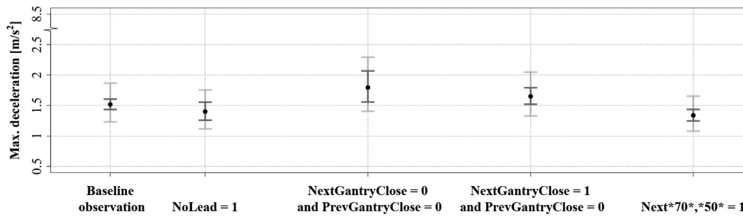
Fig. 3. Impact of the nominal explanatory variables on the maximum deceleration during the event. Black dots denote the marginal means, dark grey error bars indicate the 95% confidence intervals, and light grey error bars denote the 95% prediction intervals. The vertical axis scale is chosen based on the minimum and the maximum values available in the data. To improve the readability, the axis is interrupted at maximum deceleration equal to 2.75 m/s 2 .
