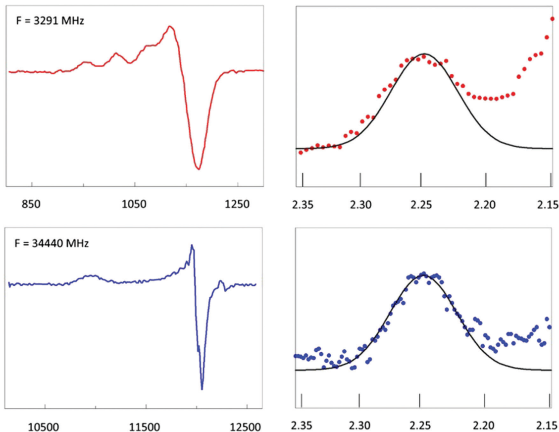
Fig. 6 EPR of spinach plastocyanin at two microwave frequencies. Red traces are S-band spectra at 3291 MHz; blue traces are Q-band spectra at 34440 MHz. The first hyperfine peak in S-band has been shifted over the hyperfine splitting, 1.5 A_z to be centralized at g_z and then plotted on the same g -value scale as the complete g_z peak of the Q-band spectrum. Their shape identity shows that inhomogeneous broadening is fully determined by a Gaussian g -strain distribution. Its extent suggests the metal site to be in an ecstatic state. Data taken from ref. 62.
