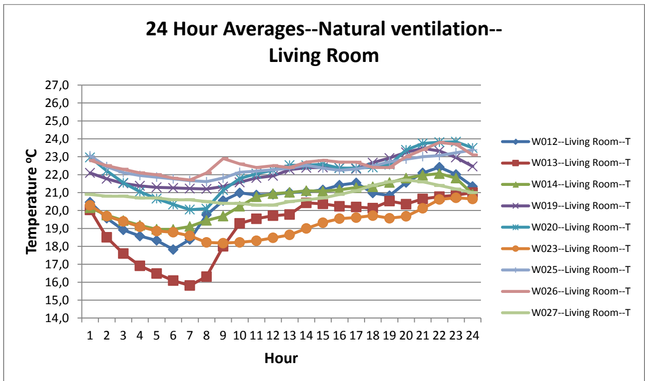
Figure 7.12: 24-hour temperature profiles for the living rooms of the naturally ventilated dwellings.
