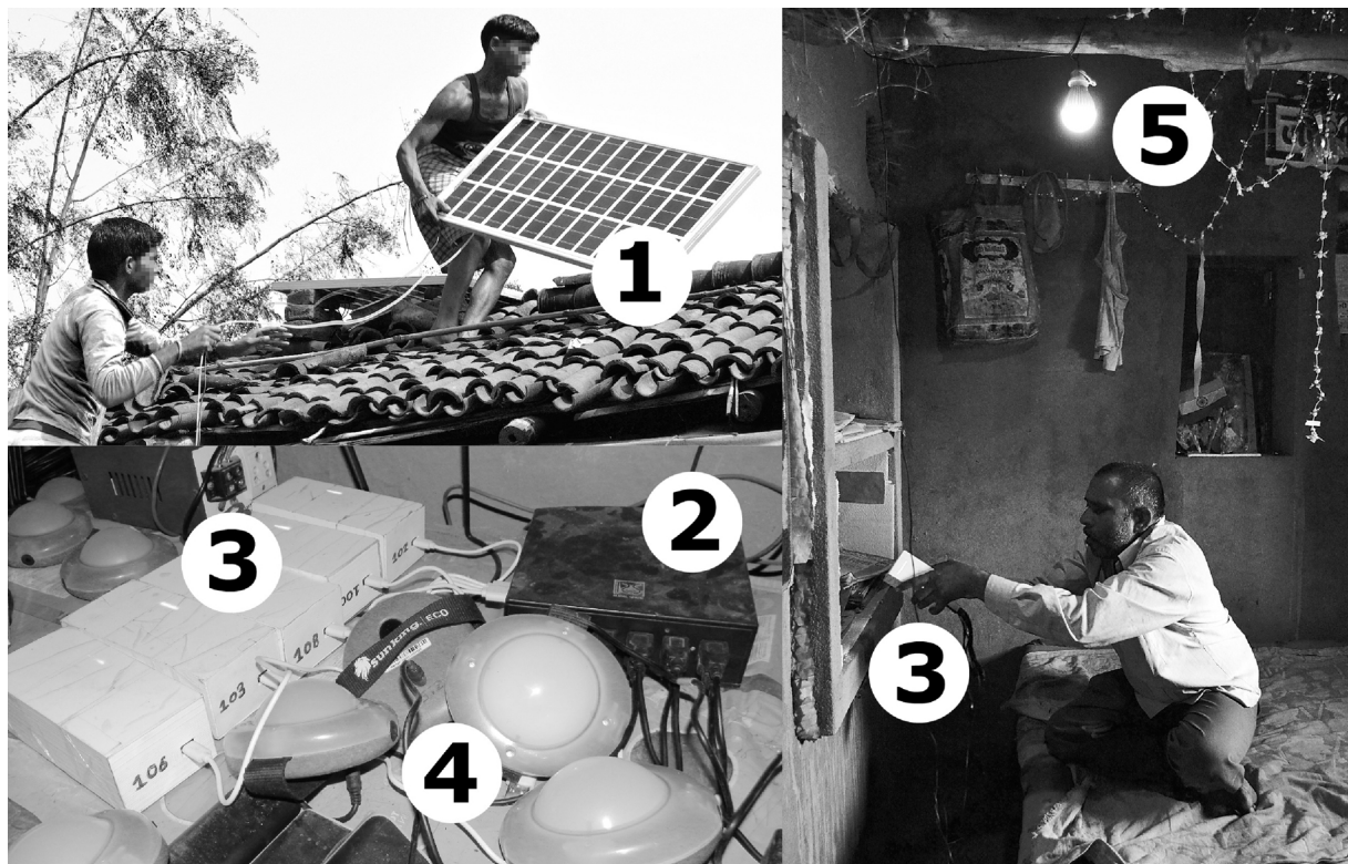
Fig. 4. Energy Distribution Infrastructure. Note the labels: '1': Solar Panel; '2': Energy Router; '3': Power banks; '4': Solar Lantern; '5': LED Bulb.
