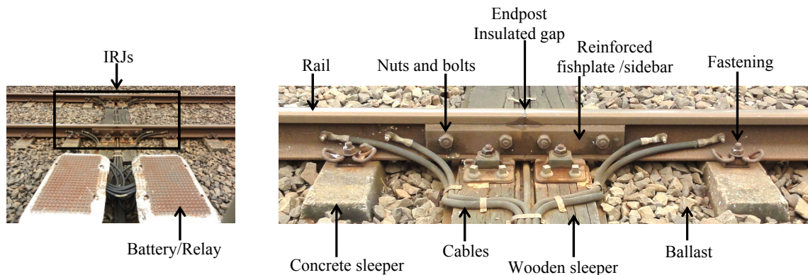
Figure 1: Picture of an IRJ and its main components.
