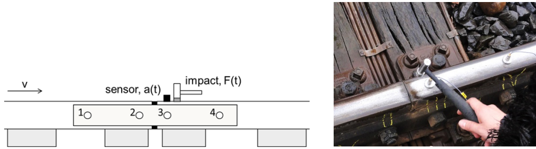
(a) A scheme of the hammer test measurement configuration
