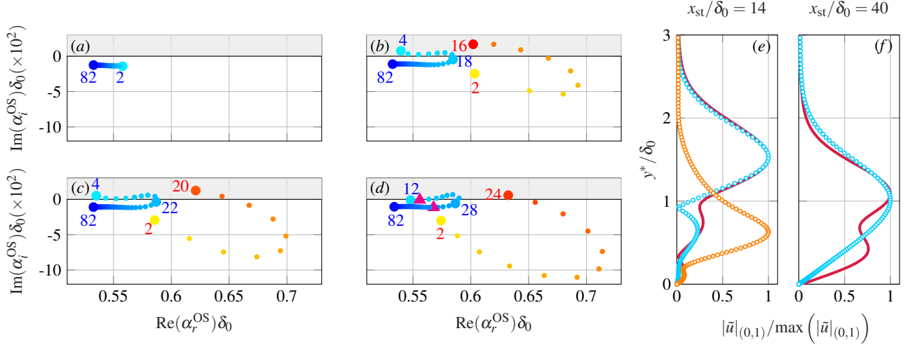
Figure 4: Trajectory of Orr-Sommerfeld eigenvalues in the range x_{\text{st}}/\delta_0 \in [2, 82] (bright-to-dark for increasing x ) for the reference no-step (a), step I (b), step II (c), and step III (d) cases. Numerals indicate x_{\text{st}}/\delta_0 locations. Orr-Sommerfeld shape functions for \beta = \beta_0 (orange and blue circles) and DNS (solid red) at x_{\text{st}}/\delta_0 = 14 (e) and 40 (f) for step III indicated by magenta triangles in (d).
