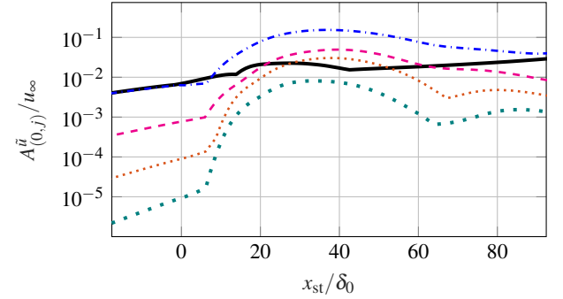
Figure 5: Evolution of the amplitude of the chordwise-velocity perturbation Fourier modes \beta = 0 (thick solid black), \beta = 2\beta_0 (dash-dotted blue), \beta = 3\beta_0 (dashed magenta), \beta = 4\beta_0 (dotted orange), \beta = 5\beta_0 (loosely dotted teal) for step III.
