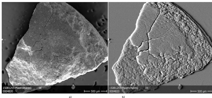
Fig. 5. Post-melting (a) Secondary Electron image and (b) Back Scattered Electron images of U_{0.5}Zr_{0.5}O_2 .
