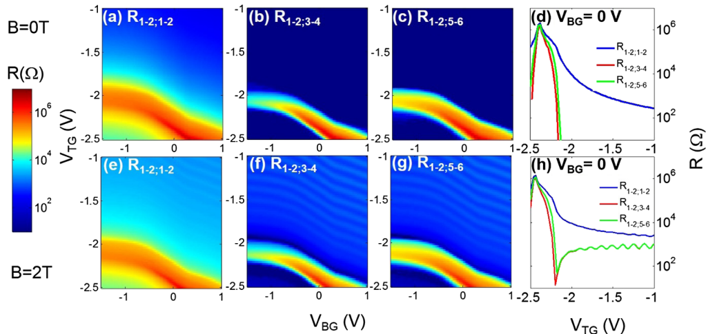
FIG. 2. Local and nonlocal resistance maps (measured at 1.8 K) at B = 0 T (a),(b),(c) and 2 T (e),(f),(g) indicating an edge conduction path at the RPs; (d) and (h) are 1D line cuts at V_{BG} = 0 V.
