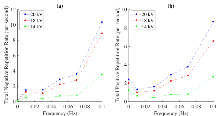
Figure 12. Frequency dependence of total PD repetition rate for (a) negative rate; (b) positive rate.
