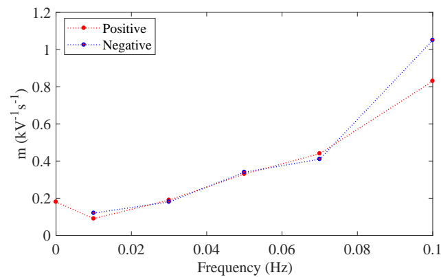
Figure 11. Frequency dependence of the voltage variation in R_{\text{tot}} .
