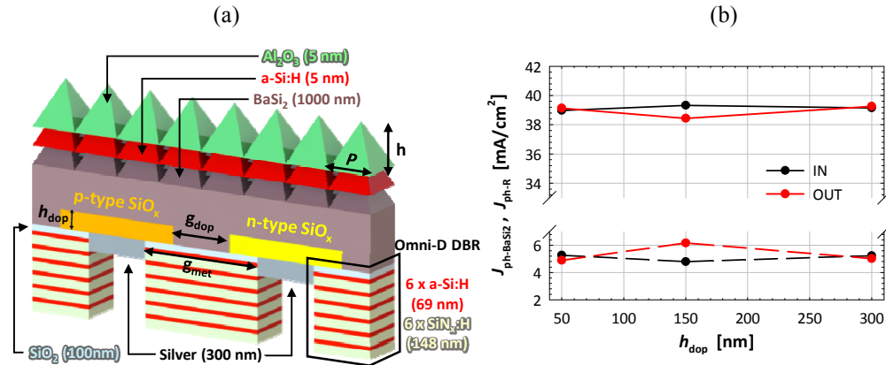
Fig. 2. (a) 3-D sketch of the back-contact BaSi 2 solar cell model. (b) Implied J_{\text{ph}} generated in the absorber (BaSi 2 ) and lost due to reflection (R), for different values of doping layers height.
