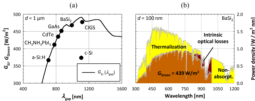
Fig. 1. (a) G_{\text{SJ}} (black line) and G_{\text{Green}} of 1- \mu\text{m} thick PV materials (black dots). (b) Power density of a 100-nm thick BaSi 2 layer, with 'Green limit' and losses indicated.
