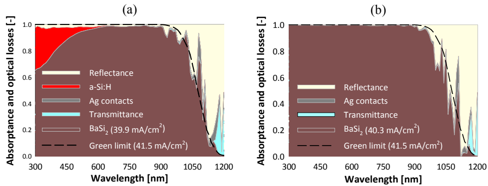
Fig. 4. Absorbance in \text{BaSi}_2 and optical losses for an architecture with \text{Al}_2\text{O}_3 + \text{a-Si:H} passivation (a) and with a 40 nm-thick \text{SiN}_x passivation (b).
