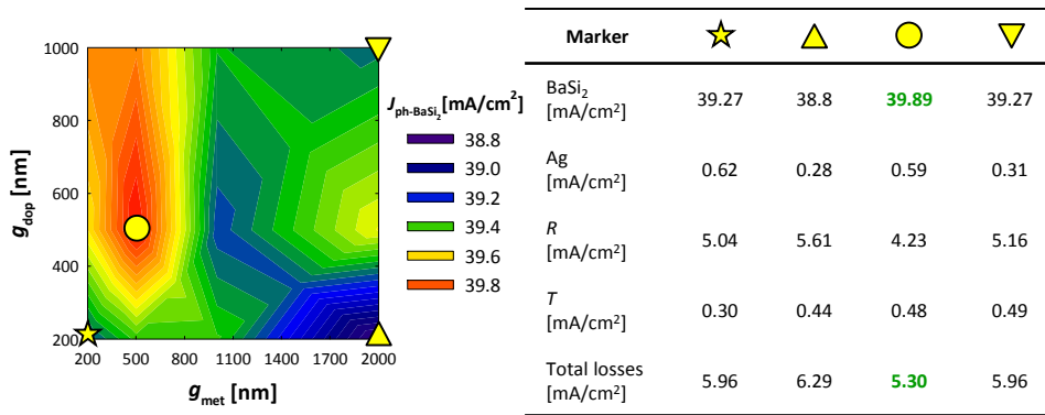
Fig. 3. J_{\text{ph-BaSi}_2} for different values of distance between doped fingers and between metal contacts (left) and breakdown of J_{\text{ph}} absorbed and lost for significant gap distances (right).
