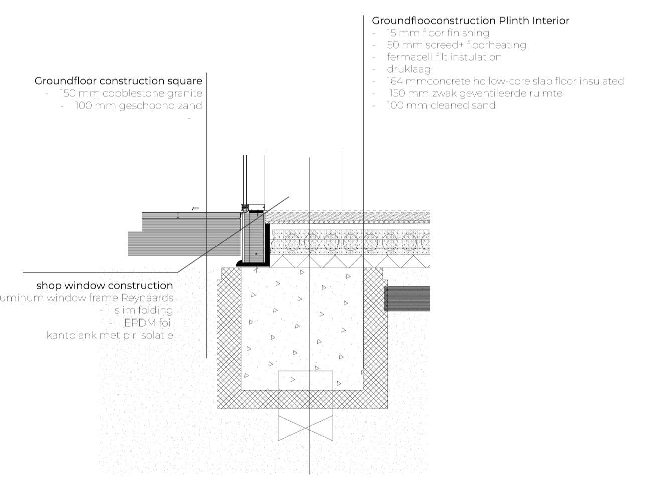
Detail 6. concrete column | facade shops
