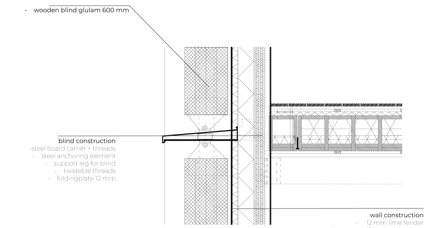
Detail 2. wooden blinds street facade
