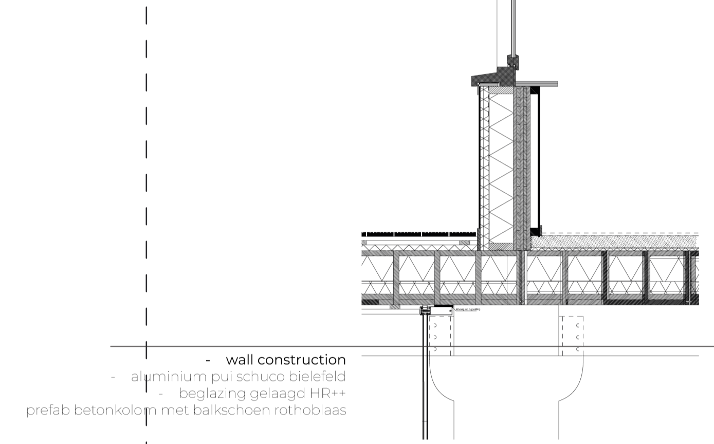
Detail 3. Floor | window | concrete column
