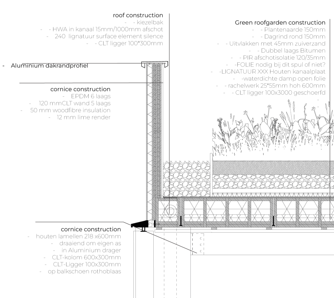
Detail 8. Green roof | Loggia ceiling
