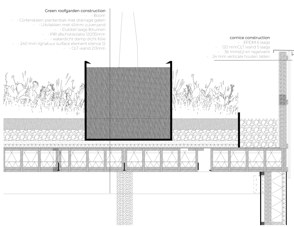
Detail 4. Green roof with planter
