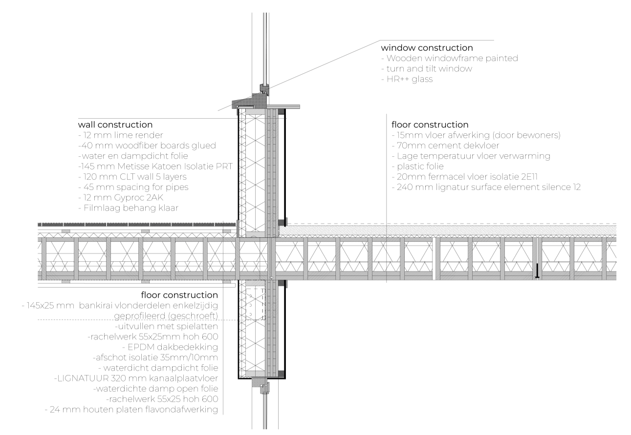
Detail 1. Window | intermediate floor
