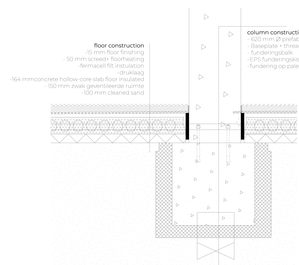
Detail 7. Concrete column groundfloor
