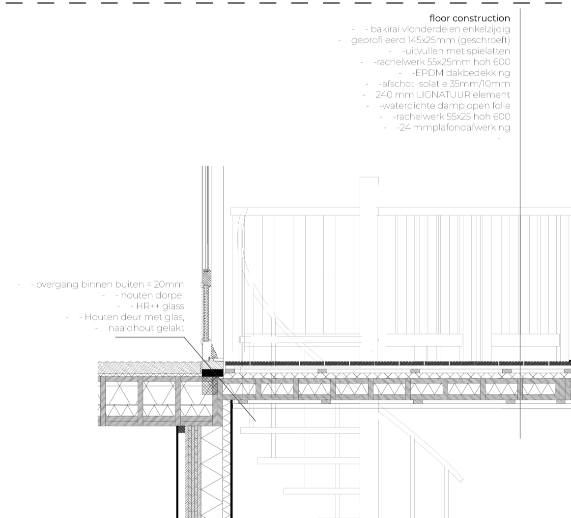
Detail 5. apartment entrance via greenalley
