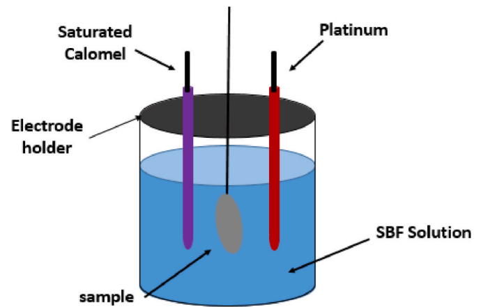
Fig. 3. The schematics of three-electrode cell used in this study for electrochemical tests.
