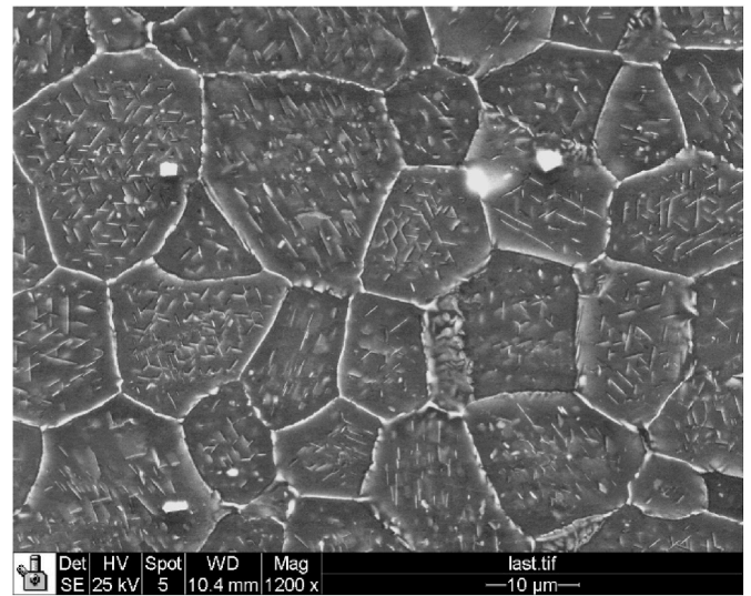
Fig. 4. Microstructure of the annealed WE43 sample prior to FSP.
