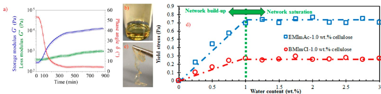
Figure 5. (a) Oscillatory time sweeps of IL solution with 5 wt % cellulose exposed to 50% RH air. (b) Solution before test and (c) material after test. (d) Yield stress of 1.0 wt % cellulose in [\text{C}_4\text{C}_1\text{im}][\text{Cl}] and [\text{C}_2\text{C}_1\text{im}][\text{Ac}] having different water contents [Reprinted with permission from ref 119. Copyright 2017. American Chemical Society].
