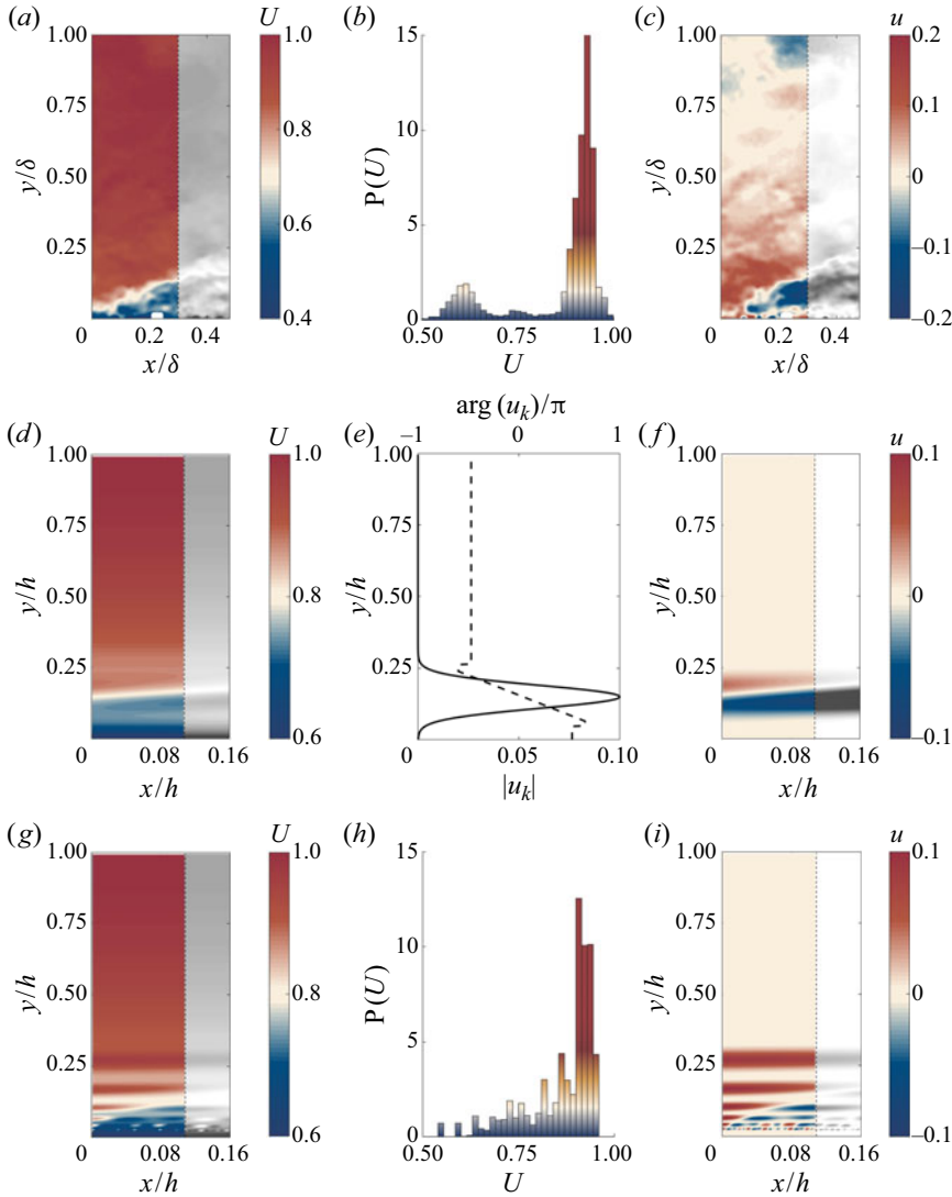
Figure 2. Instantaneous velocity fields. Data from E1 ( a–c ), N1M1 ( d–f ) and N2M6 ( g–i ). Panels ( a,d,g ) and ( c,f,i ) show the full and fluctuating velocity fields, U and u , respectively. Panels ( b,h ) show the corresponding p.d.f. while the amplitude and phase profile of the individual mode is shown in panel ( e ). The region of the fluctuating and full fields shown in colour denotes the streamwise extent used for the construction of the p.d.f., \mathcal{L}_x^+ = 1590 for all datasets.
