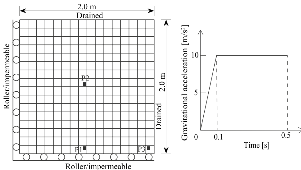
Fig. 11 Layout of the 2D slumping block problem and corresponding application ramp for the gravitational acceleration
