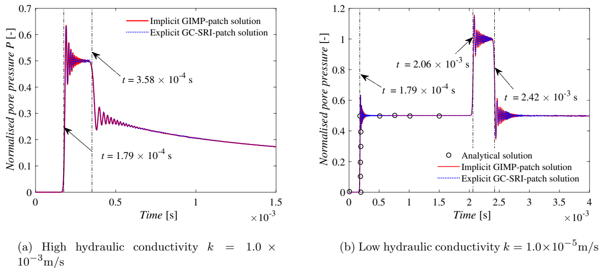
Fig. 8 Propagation of a shock pressure wave: comparison between analytical and MPM (implicit GIMP-patch and explicit GC-SRI-patch) solutions
