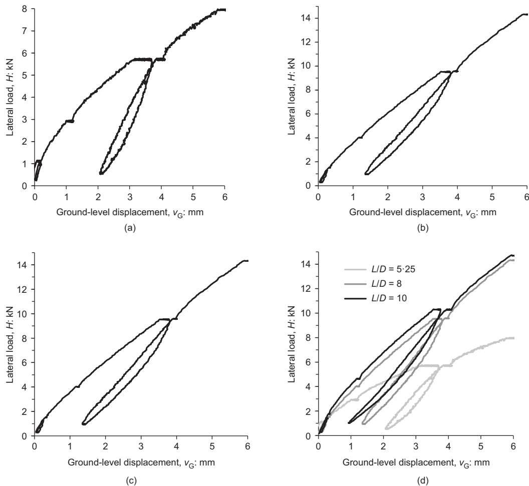
Fig. 5. Comparison of load–displacement response for D = 0.273 m diameter piles with different length-to-diameter ratios during initial load stages 1–4: (a) L/D = 5.25 (DS1); (b) L/D = 8 (DS3); (c) L/D = 10 (DS4); (d) three L/D ratios
