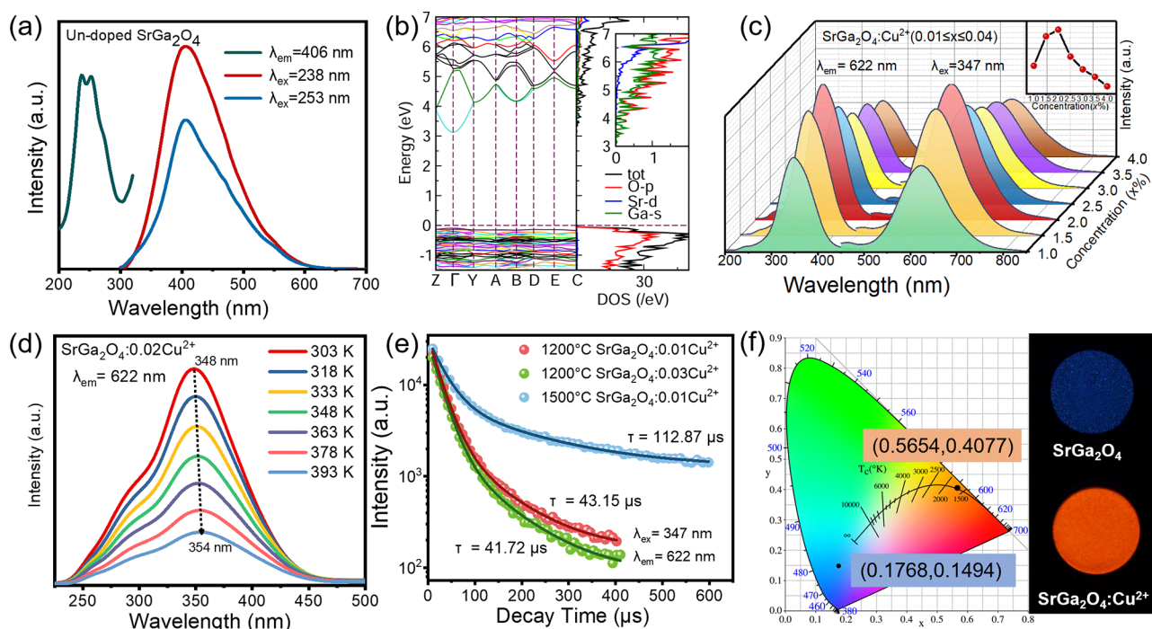
Figure 2. Excitation and emission spectra of (a) \text{SrGa}_2\text{O}_4 and (c) \text{SrGa}_2\text{O}_4:\text{xCu}^{2+} ( x = 0.01, 0.015, 0.02, 0.025, 0.03, 0.035, and 0.04 ). The inset in (c) shows the dependence of the integral emission intensity on the concentration of Cu ions ( x ). (b) Electronic structure of \text{SrGa}_2\text{O}_4 without \text{Cu}^{2+} dopant or intrinsic defects. The inset is the enlarged density of states for the bottom of the host conduction band. (d) Temperature dependence of excitation spectra for the \text{SrGa}_2\text{O}_4:0.02\text{Cu}^{2+} phosphor. (e) Luminescence decay curves of \text{SrGa}_2\text{O}_4:\text{xCu}^{2+} ( x = 0.01 and 0.03 ) sintered at 1200^\circ\text{C} and \text{SrGa}_2\text{O}_4:0.01\text{Cu}^{2+} sintered at 1500^\circ\text{C} . (f) Chromaticity coordinate diagrams (CIE) of luminescent \text{SrGa}_2\text{O}_4 and \text{SrGa}_2\text{O}_4:0.02\text{Cu}^{2+} and their photographs.
