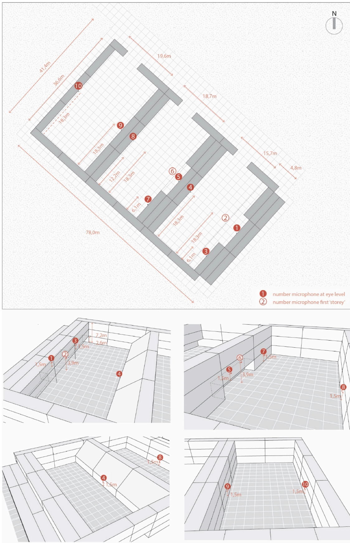
Fig. 5. Top view and closeups of the courtyards and microphone positions.
