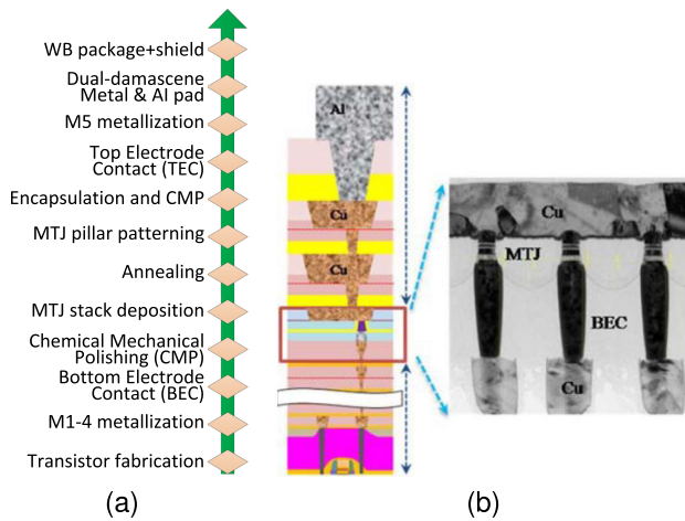
FIGURE 4. General manufacturing process of STT-MRAM: (a) bottom-up processing flow of STT-MRAM cells, (b) vertical cross-section structure of STT-MRAM cells [27].
